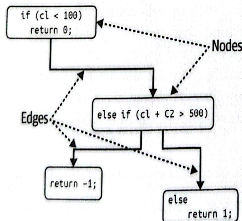
Figure 6-1. Cyclomatic Complexity graph for the decision function
